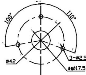
H2N/H4N Flange mount holes
